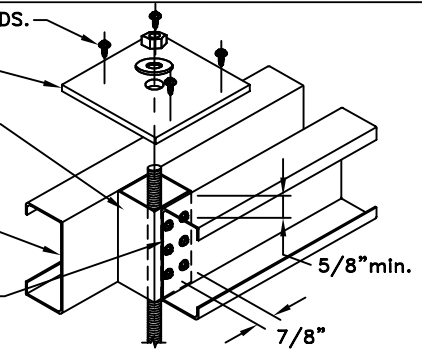
Hanger Rod Assembly Detail
